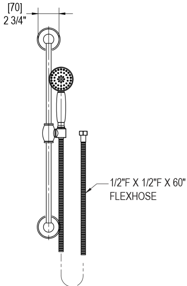
ADJUSTABLE SLIDE BAR WITH HAND HELD SHOWER ASSEMBLY
