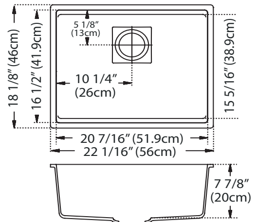
Dimensional Drawing
