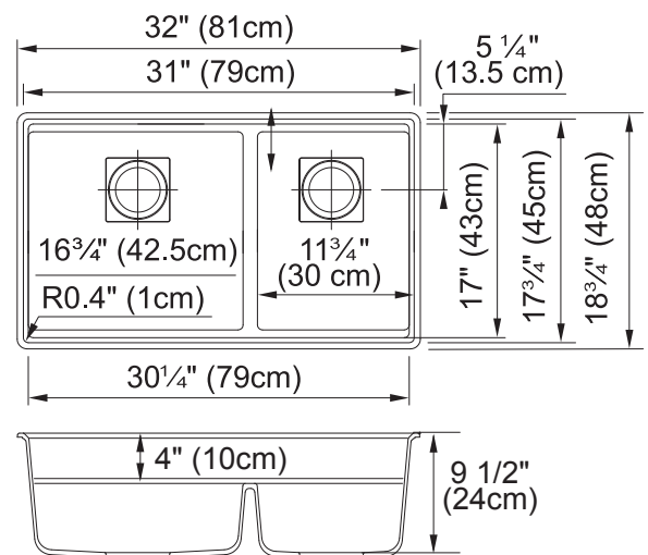
Dimensional Drawing
