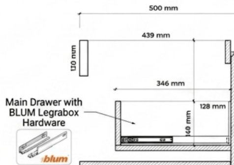
CROSS-SECTIONAL VIEW
